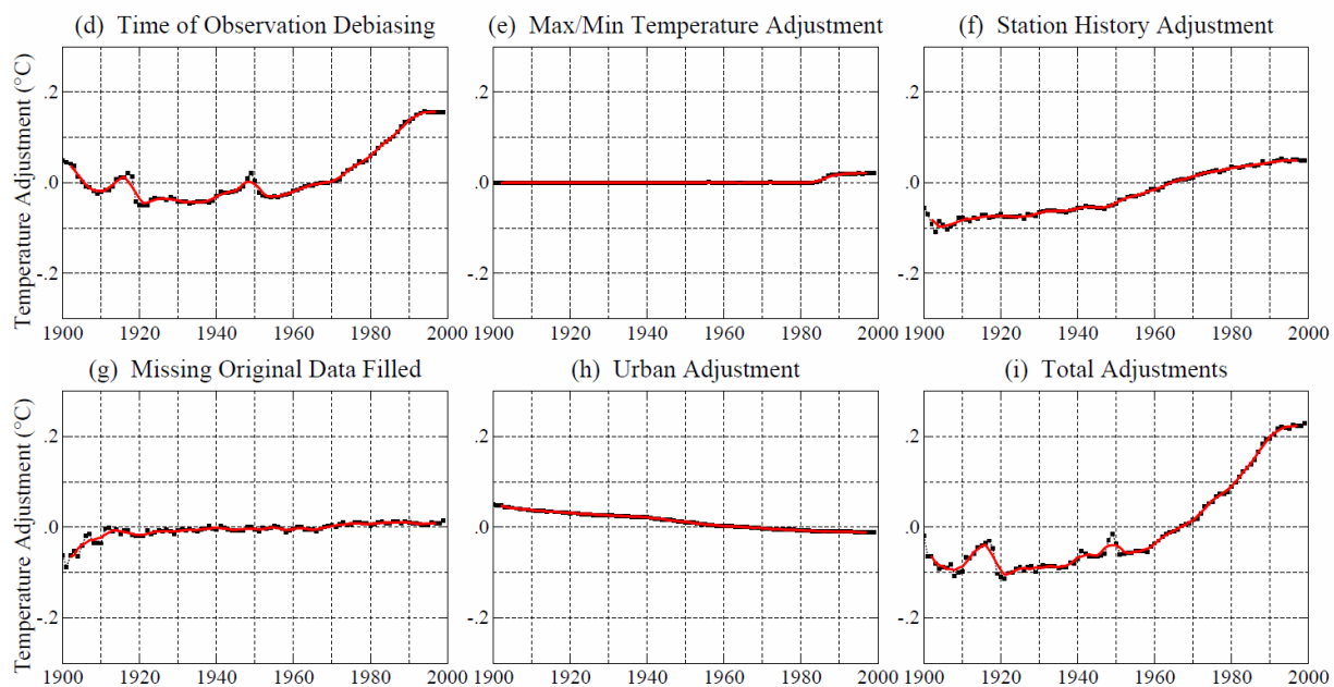
Figure 9. USHCN corrections (2001)
